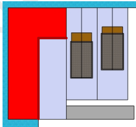
Figure 4.25(A)(4)b: Point or Peninsula
