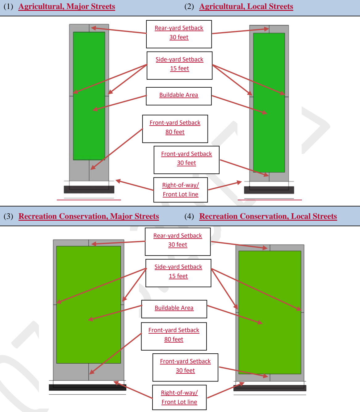
Figure 4.25(A): Minimum Yard Setbacks
